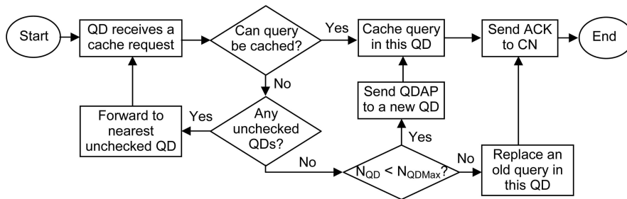
Fig. 2. Procedure for caching queries in QDs.
