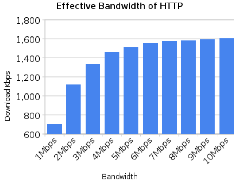
Figure 1. Effective Bandwidth of HTTP
